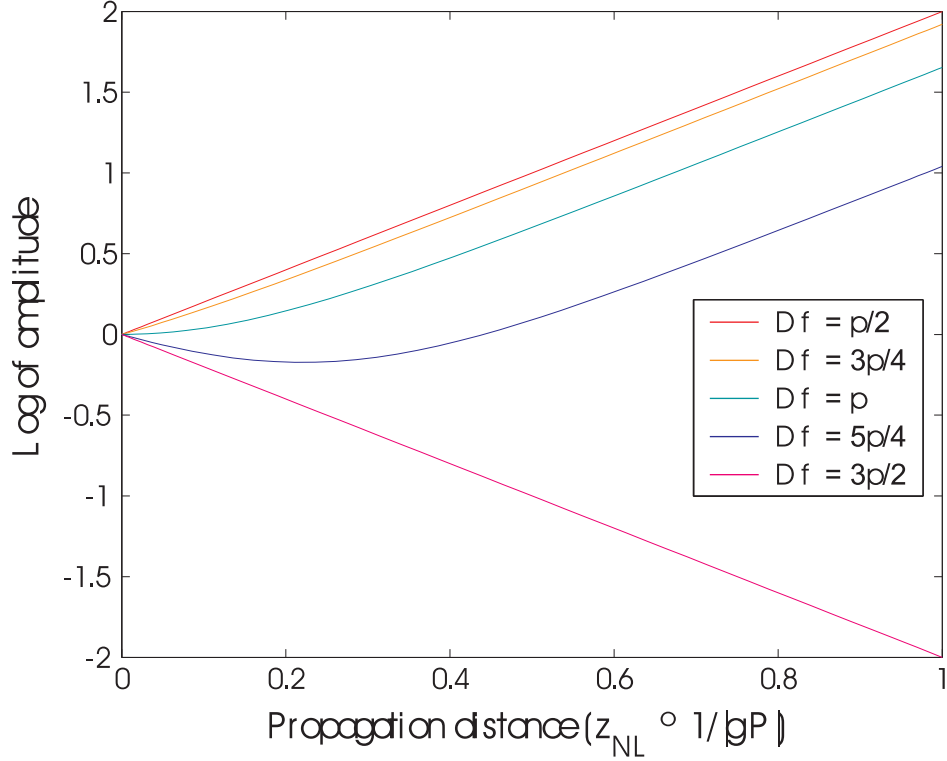
FIG. 3: Logarithm of signal beam amplitude as a function of propagation distance.
